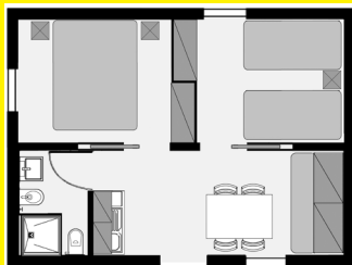
Bungalow Confort 4+1
